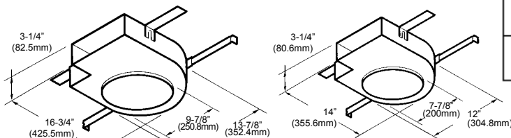
MODEL 503 HOUSING
